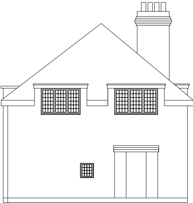
West Elevation Existing
